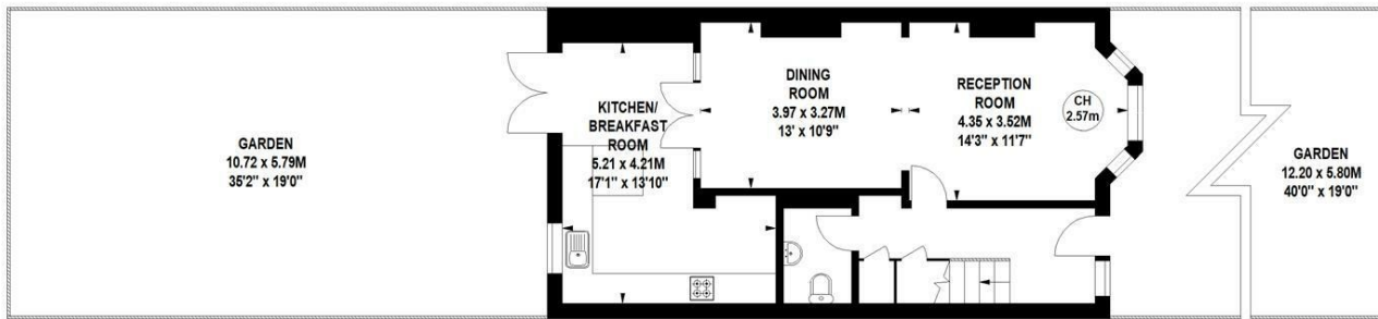
Ground Floor
